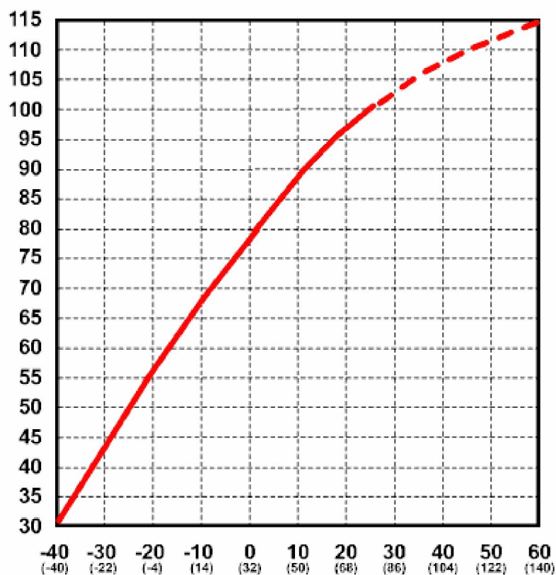
CAPACITY vs. TEMPERATURE °C
